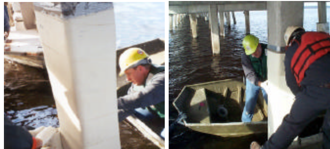
Figure 6. Aquawrap® installation
